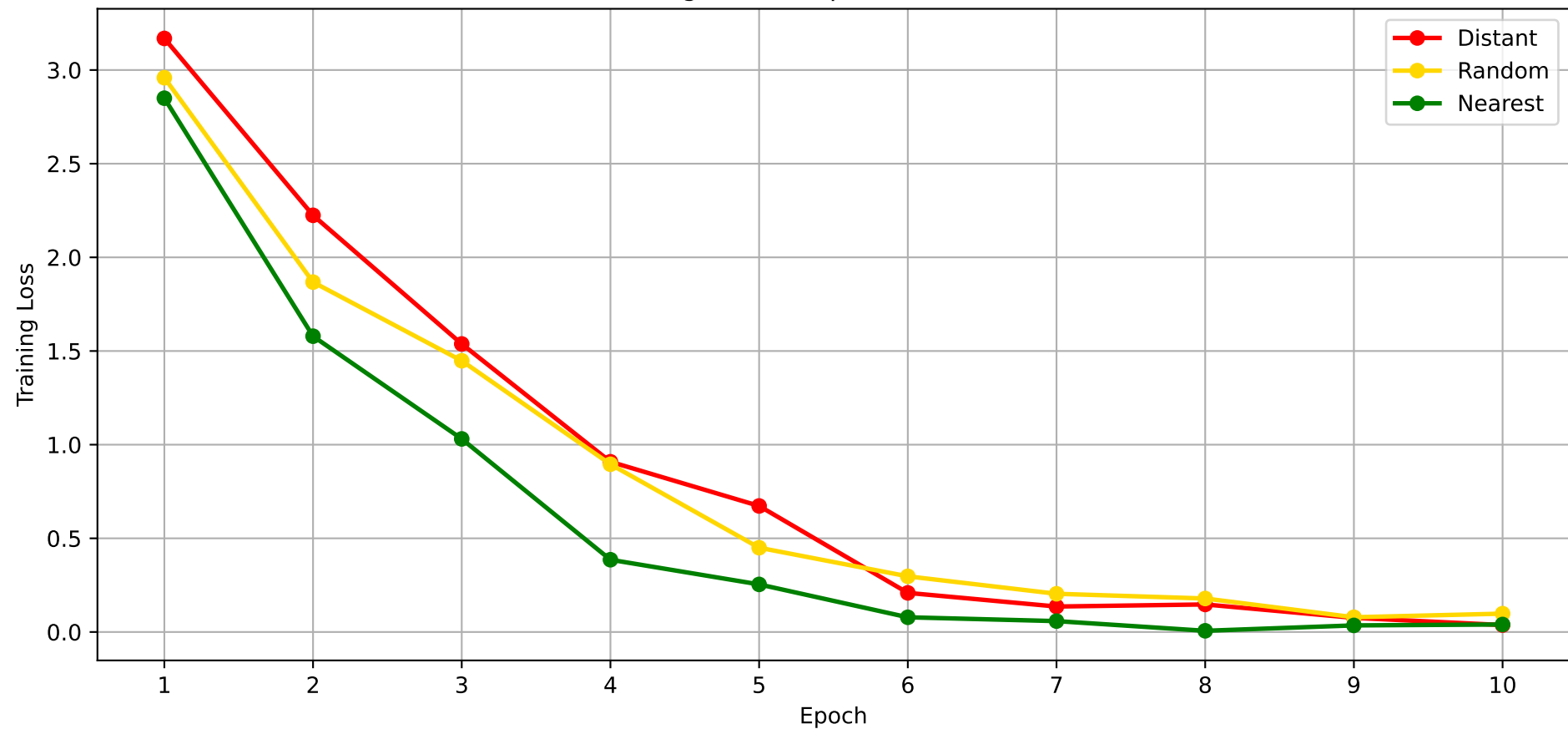
Training Loss vs Epoch (Select 25%)
