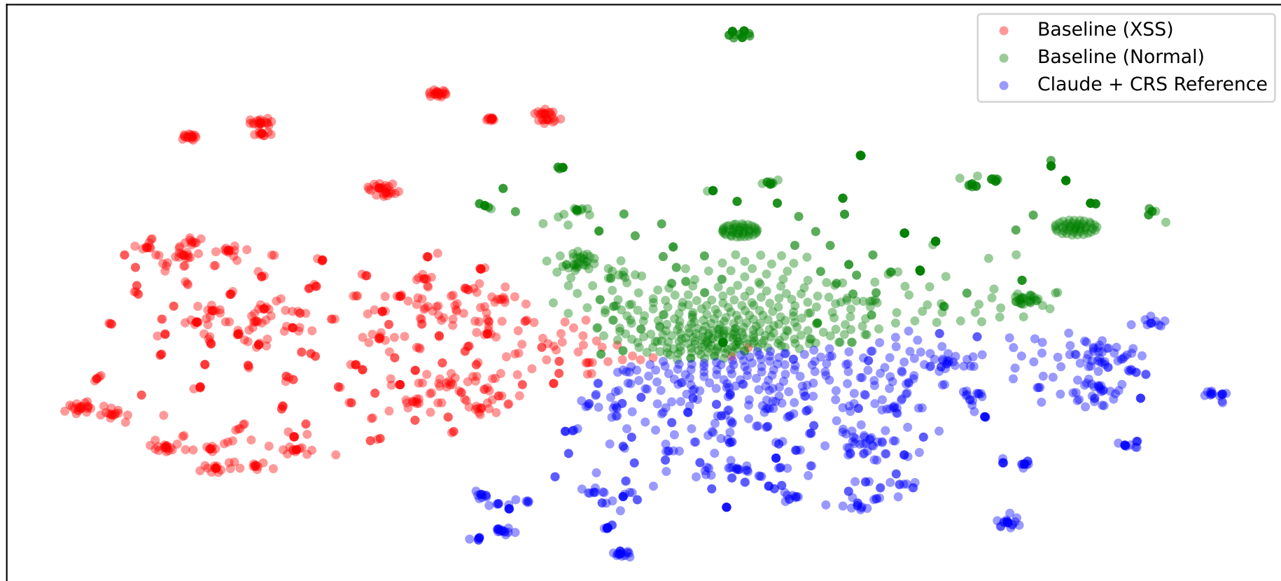
XSS Payload Distribution (Char-TFIDF + t-SNE)
