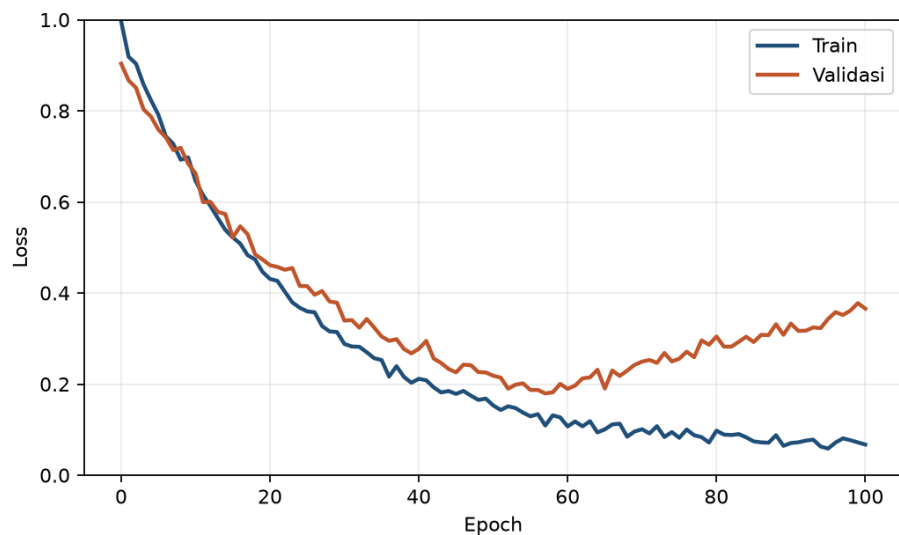
Gambar 6: Gambar 5.1 - Learning curve klasik overfit
