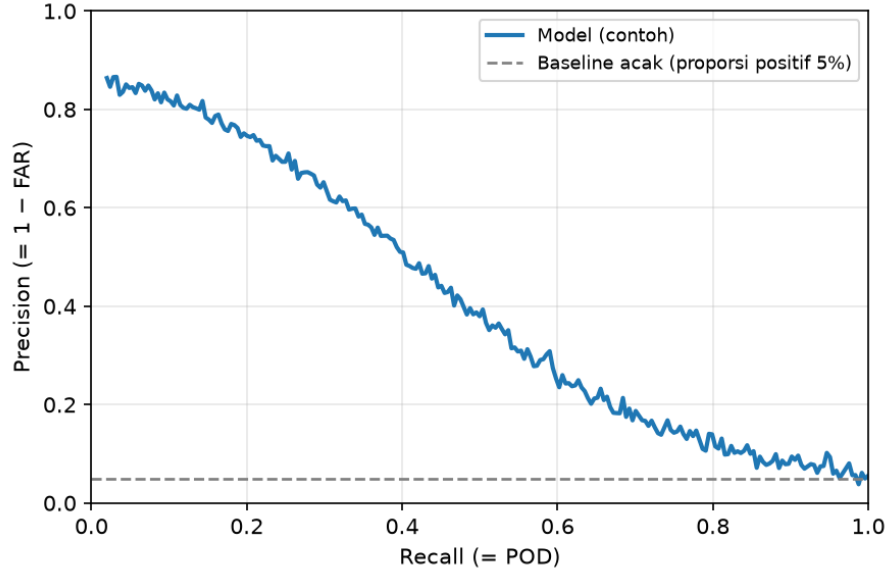
Gambar 12: Gambar 9.1 - Precision-recall curve
