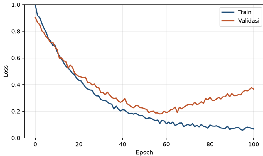
Gambar 5: Gambar 4.1 - Contoh learning curve overfit
