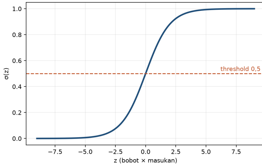
Gambar 3: Gambar 3.1 - Kurva sigmoid
