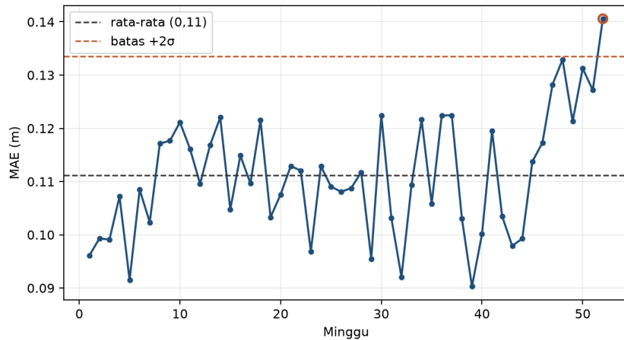
Gambar 14: Gambar 10.1 - Grafik kendali metrik operasional
