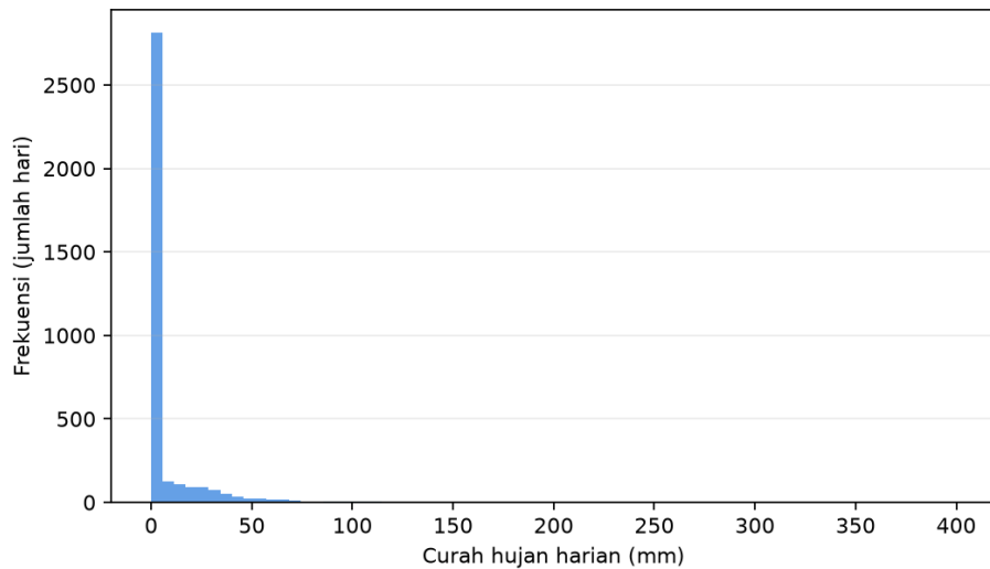
Gambar 7: Gambar 6.1 - Distribusi curah hujan harian
