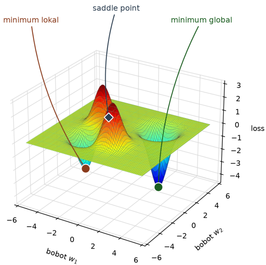
Gambar 8: Gambar 4.2 - Permukaan loss landscape dua bobot
