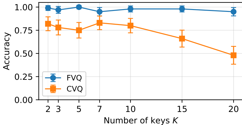
Gemma-3-4b-it — vary K at N = 10
