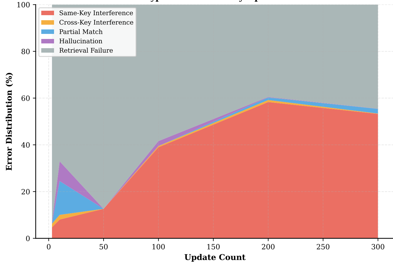
Error Type Distribution by Update Count
