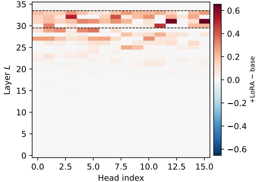
(b) Attention routing — \Delta P(\text{attend } v_{\text{last}})
