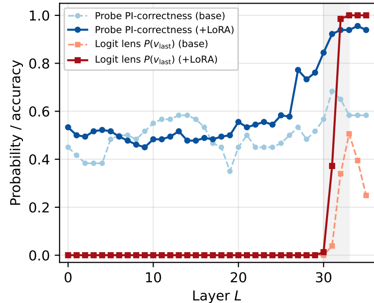
(a) Probing \&amp; logit lens
