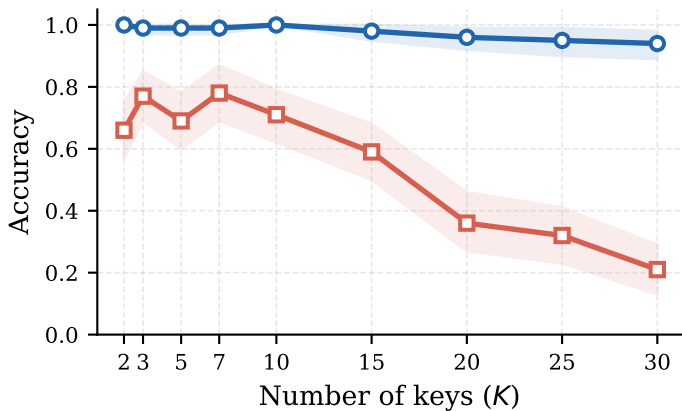
Varying key count ( N = 10 fixed)
