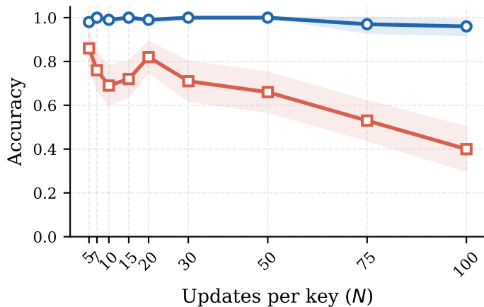
Varying update depth ( K = 5 fixed)
