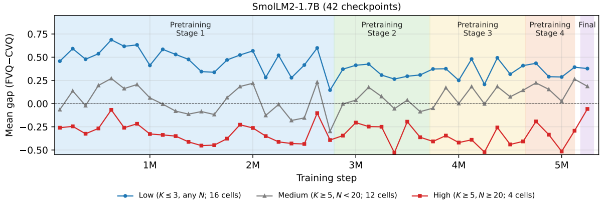
Figure 12: Mean FVQ–CVQ gap on Arbitrary-Single across the SmolLM2-1.7B (Ben Allal et al., 2025) training trajectory, under the same three-bin partition as Figure 4. Coloured bands mark the four documented pretraining stages plus the released final model.
