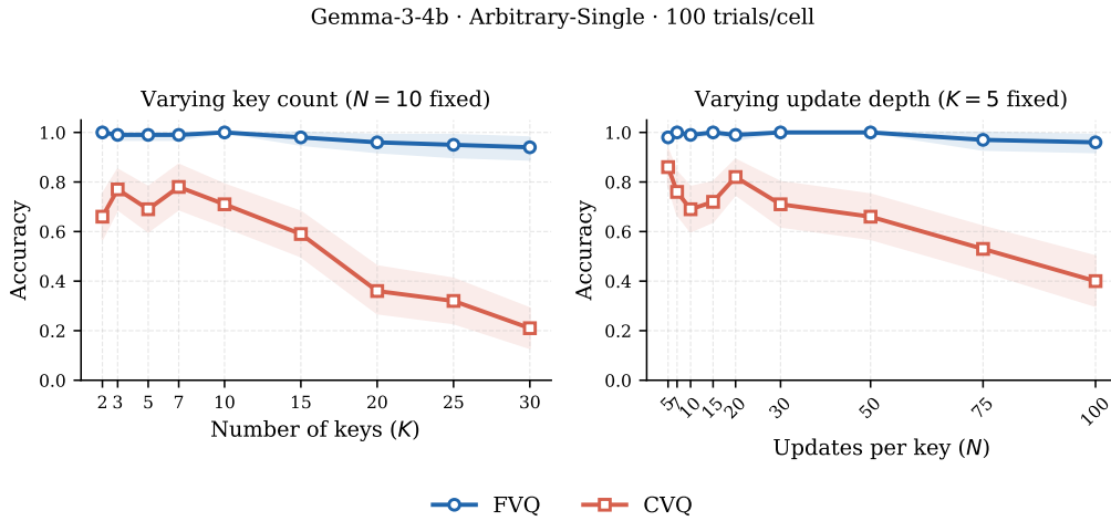
Figure 11: Baseline FVQ and CVQ accuracy on Gemma-3-4b-it across the unified grid. Clean primacy regime (FVQ \gg CVQ) at every cell, in contrast to Qwen2.5-3B-Instruct which crosses into the reversal regime at high stream load. The LoRA recovery in Tables 15 and 16 closes this gap on all 28 held-out cells.
