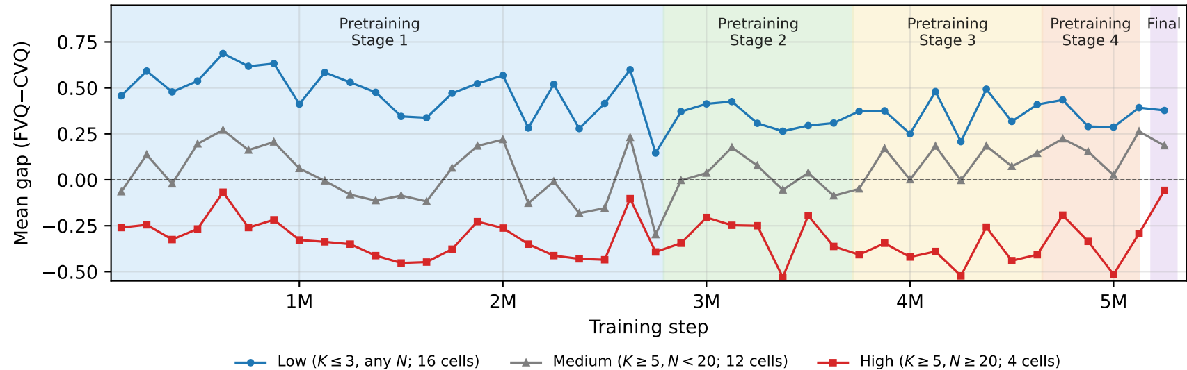
SmolLM2-1.7B (42 checkpoints)
