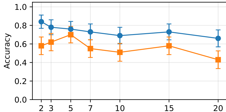
Gemma-3-4b-it --- vary K at N = 10
