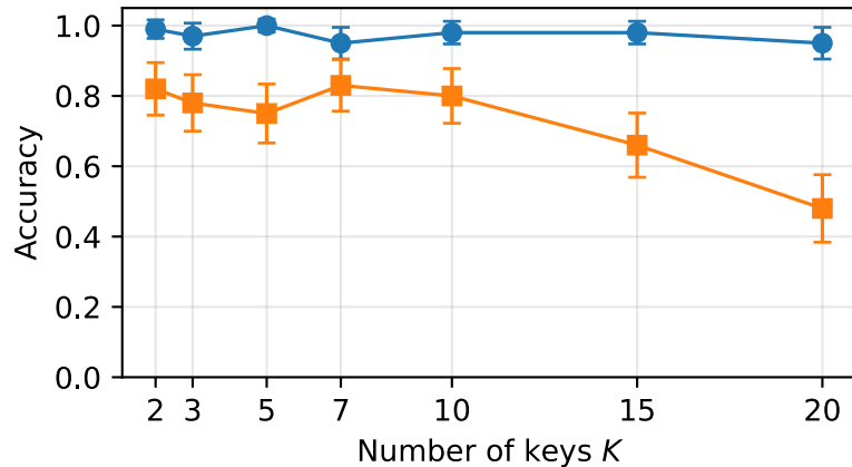
Gemma-3-4b-it --- vary K at N = 10
