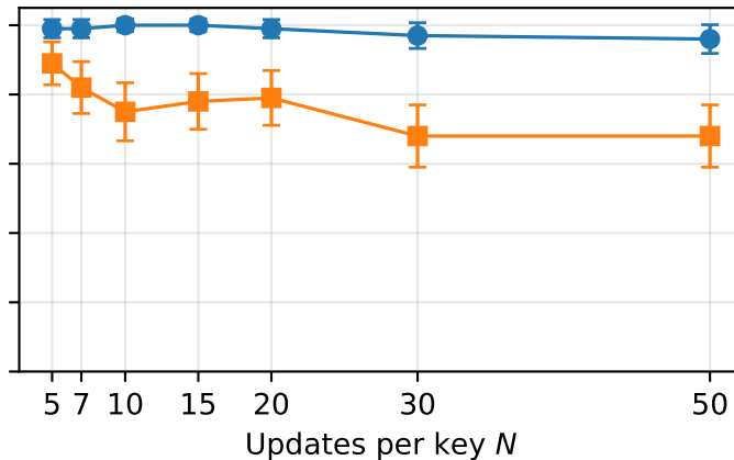
Gemma-3-4b-it --- vary N at K = 5
