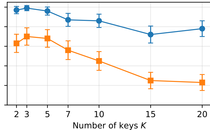
Gemma-3-4b-it --- vary K at N = 50
