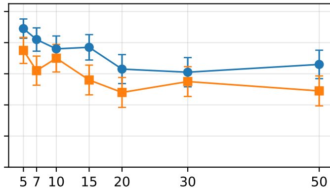
Gemma-3-4b-it --- vary N at K = 5
