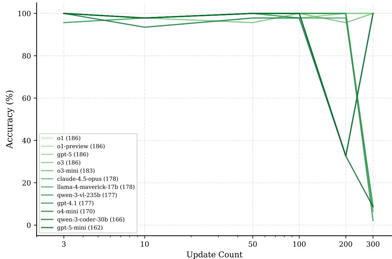
Top 12 Models (Highest RIES)
