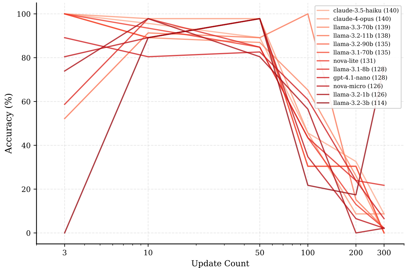
Bottom 12 Models (Lowest RIES)
