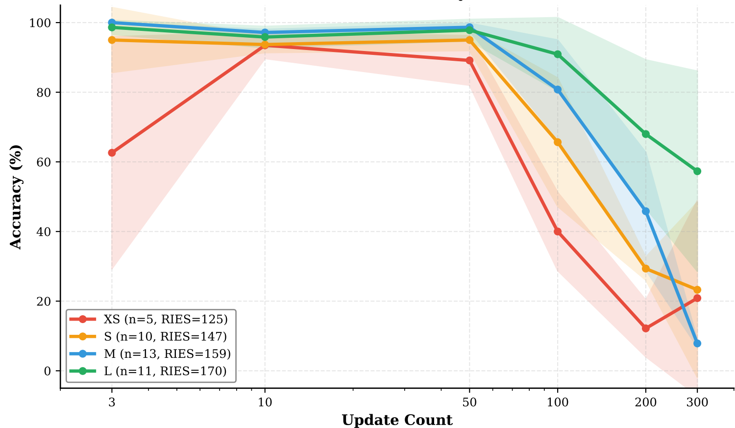
Retroactive Interference by Model Size
