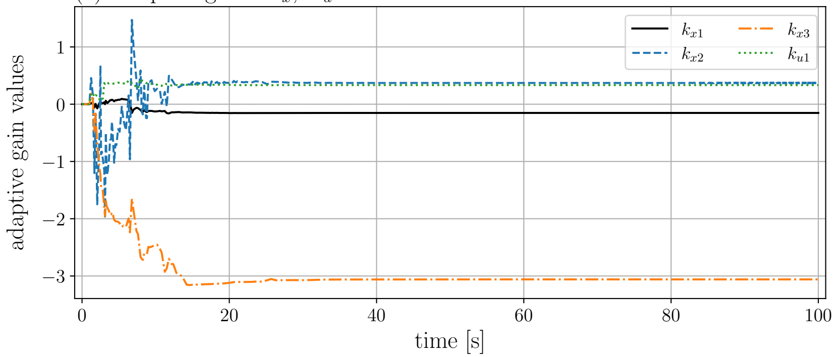
(2) Adaptive gains K_x, K_u
