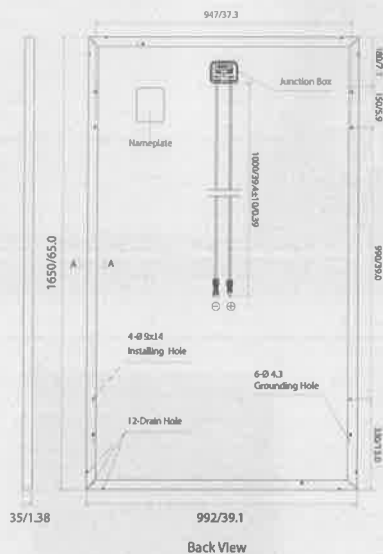
DIMENSIONS OF PV MODULE (mm/inches)
