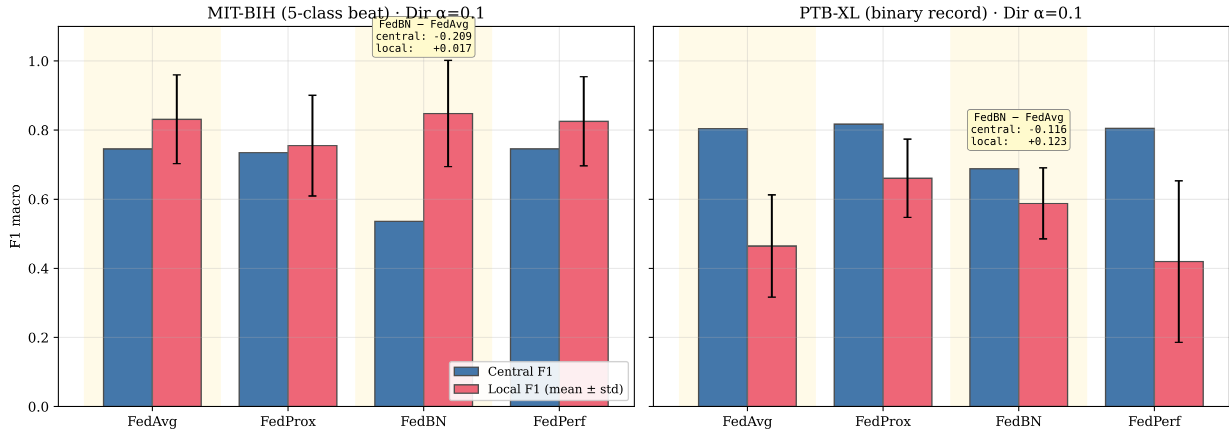
Cross-task validation: FedBN ranks below FedAvg on central but above on local — both datasets (no-DP, Dir \alpha=0.1 )
