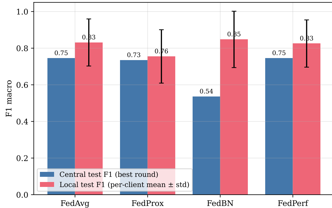
Dirichlet \alpha=0.1
