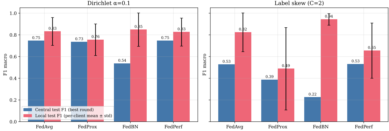
Fig. 1. Central vs. per-client local macro F1 across the four aggregations on MIT-BIH, for Dirichlet \alpha=0.1 (left) and label skew C=2 (right). Blue bars are central F1; red bars are local F1 (mean \pm std). Under each partition FedBN has the lowest central F1 but the highest local F1 — the eval-regime flip.
