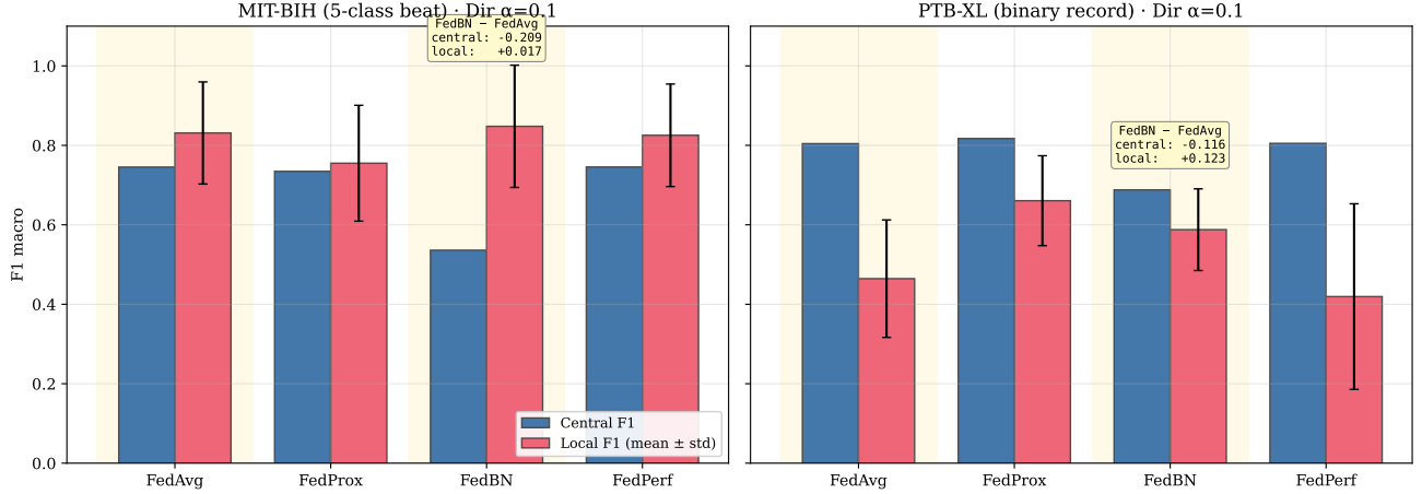
Fig. 3. Cross-task summary (Dirichlet \alpha=0.1 , no DP). Both datasets show FedBN central F1 (blue) below FedAvg and FedBN local F1 (red) above FedAvg. The eval-regime flip in FedBN–FedAvg is task-agnostic: -0.209 central / +0.017 local on MIT-BIH, -0.116 central / +0.123 local on PTB-XL.
