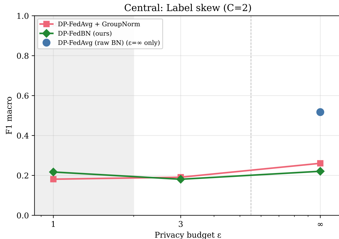
DP-FedBN preserves local-eval advantage under DP on label-skew, mixed on Dirichlet \alpha=0.1
