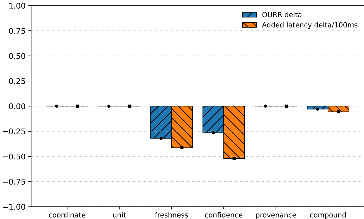
Delta Proposed-Strict
