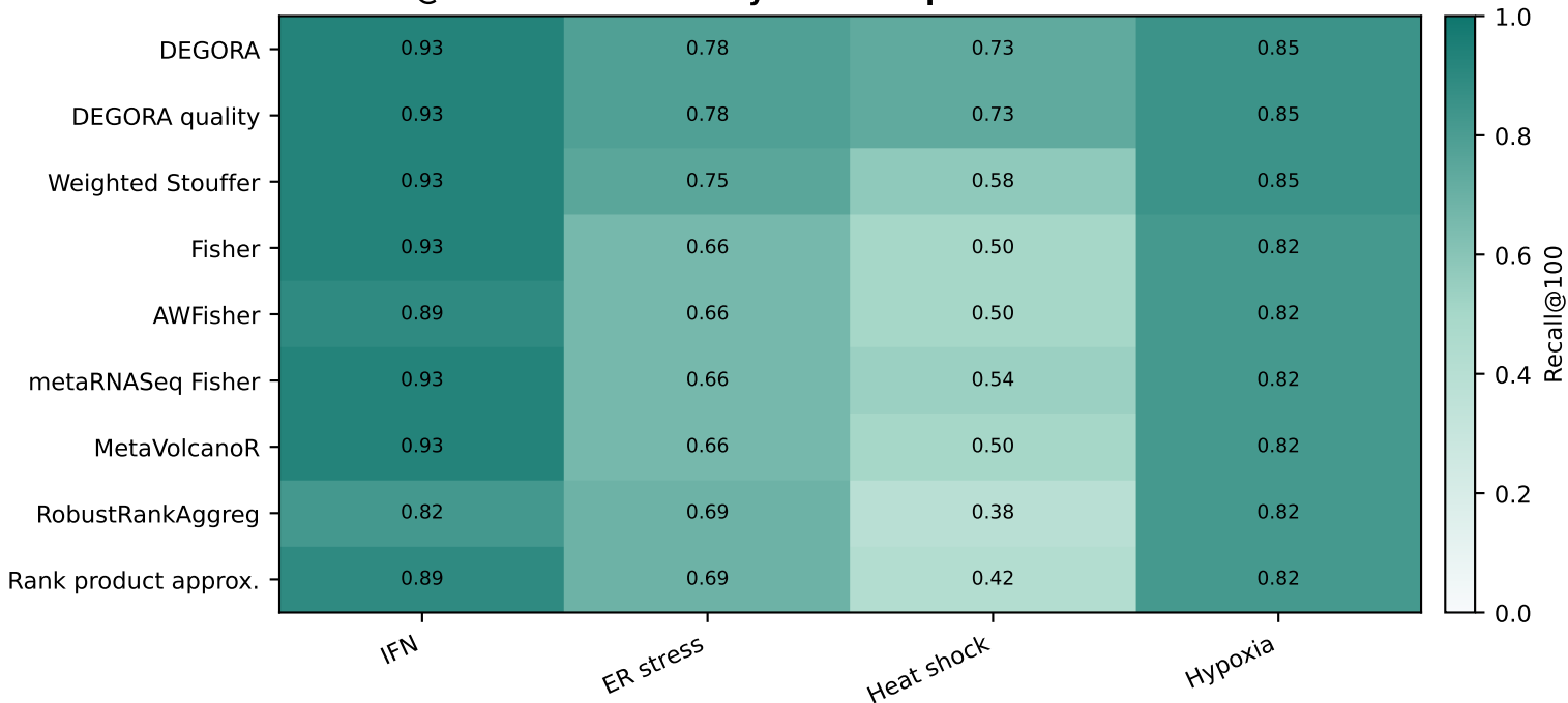
B. Recall@100 versus summary-level comparators
