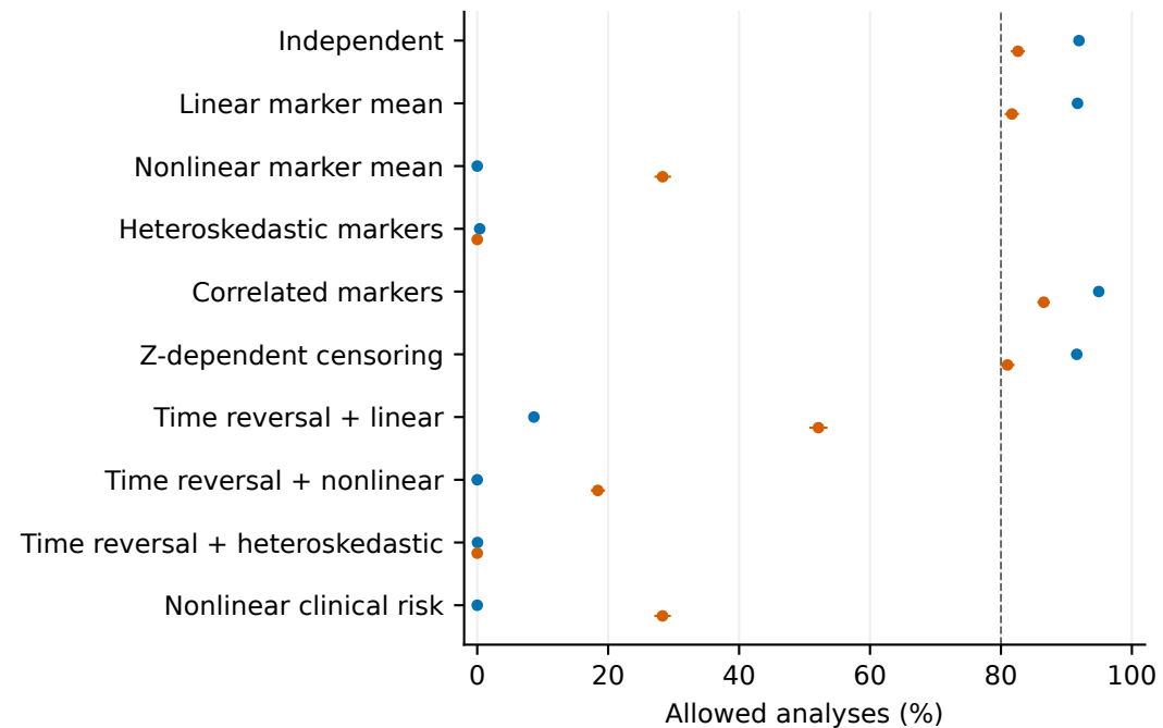
C Normal and unsuitable analyses retained
