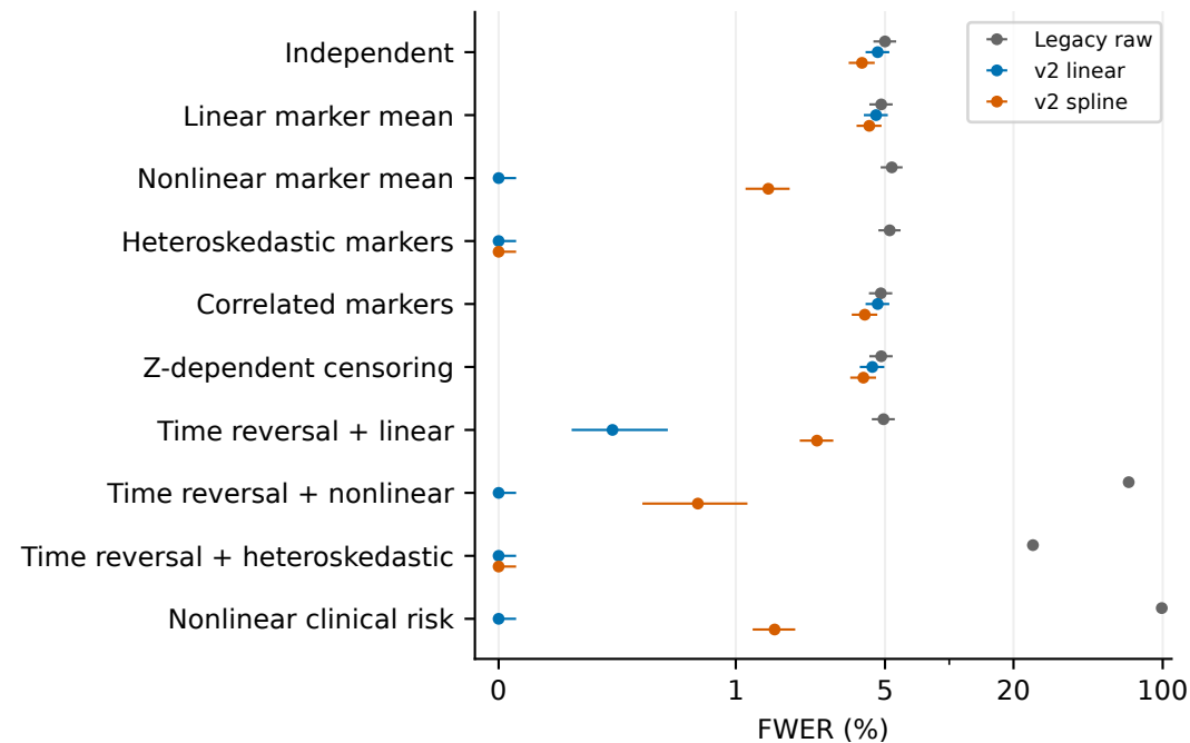
A Raw and reported errors
