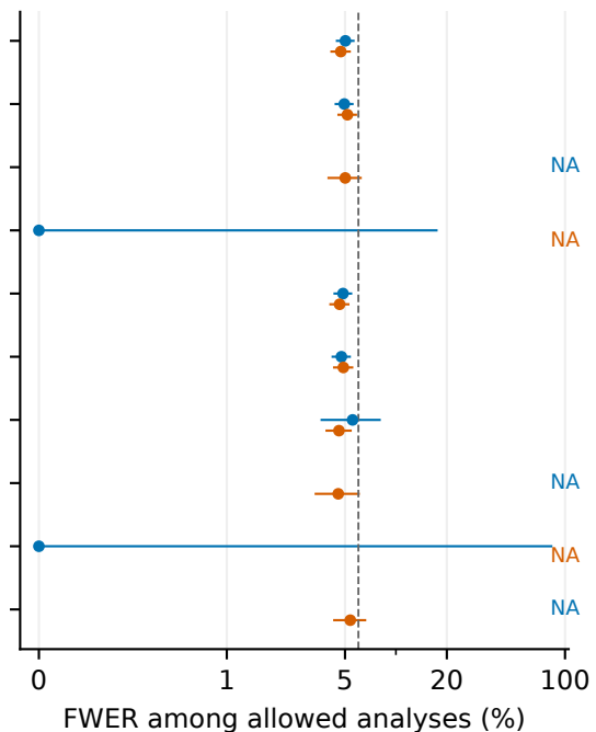
B Errors among allowed analyses
