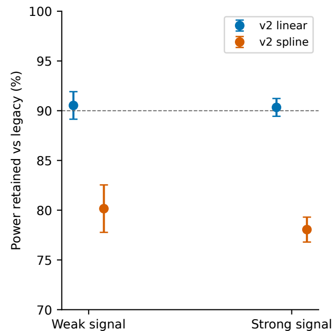
D Partial-null power retention
