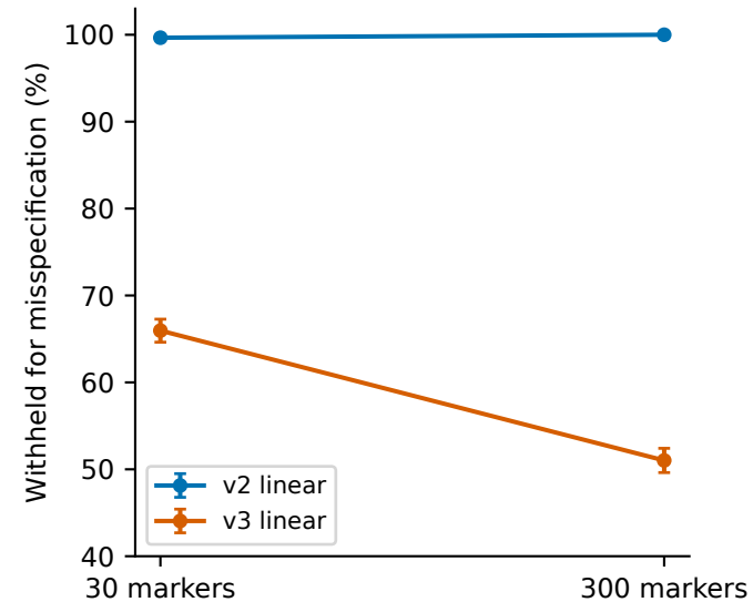
B Missed heteroskedasticity increases
