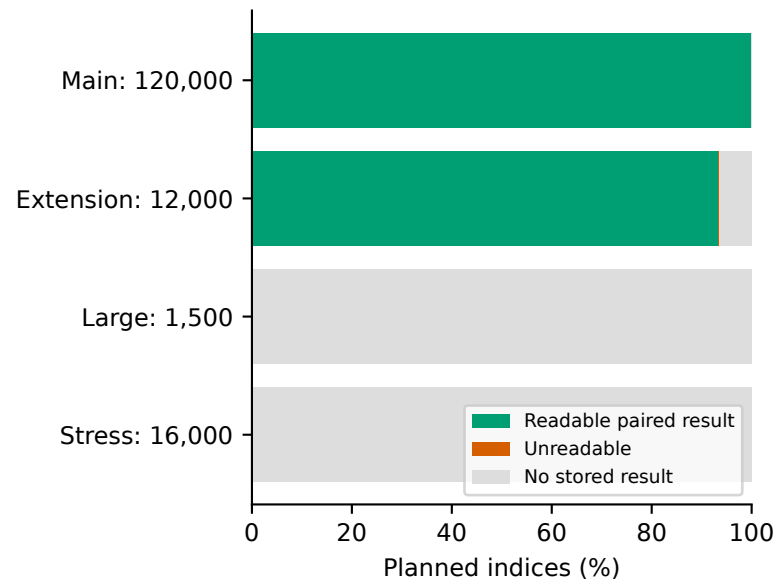
D Confirmation remains incomplete
