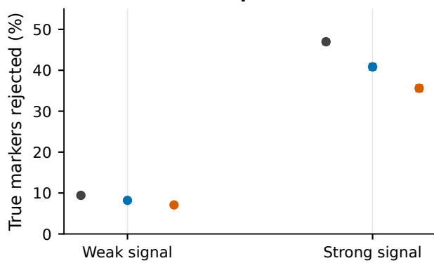
A Power over all planned datasets
