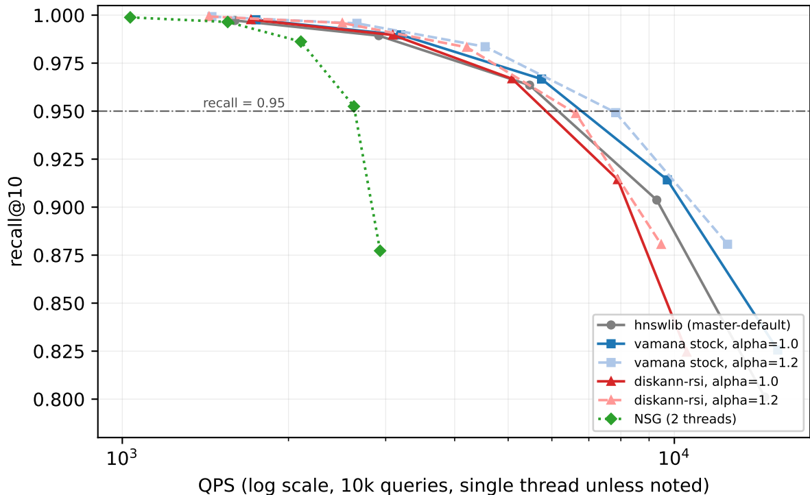
SIFT1M: recall@10 vs QPS, one machine, one protocol
