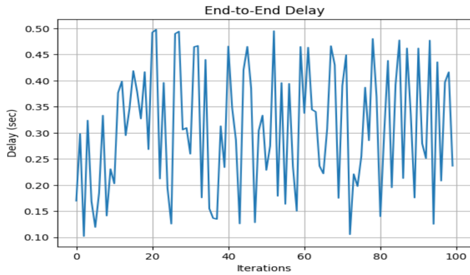
Figure 5: End-to-end delay
