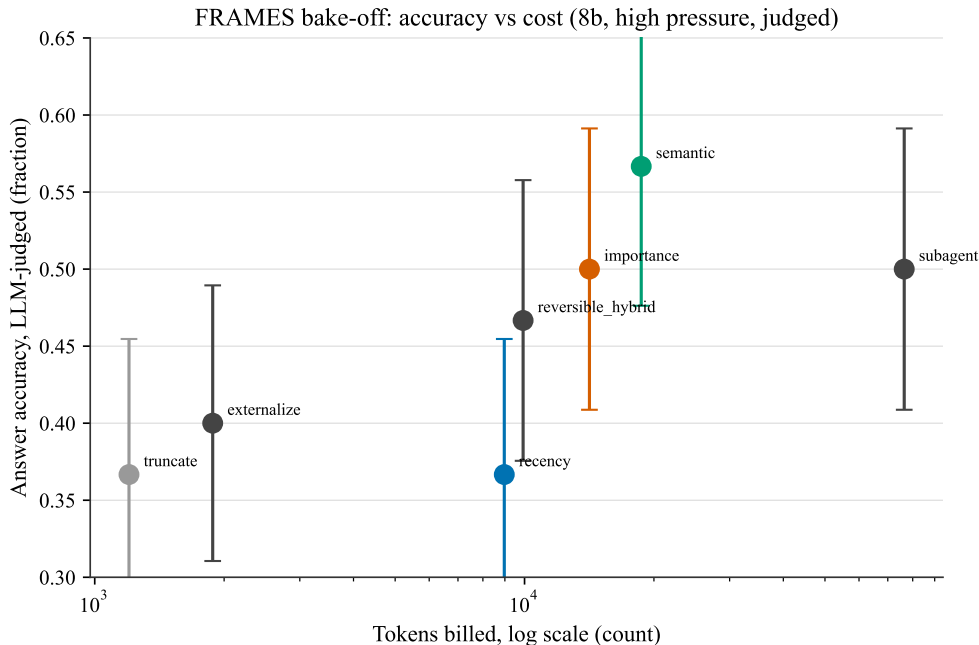
Figure 2: Accuracy versus cost on FRAMES under pressure (EXP-003b, 8B, n=30 ). The structure- and retrieval-preserving policies sit on the cost-quality frontier; recency (the shipped default) and sub-agent are dominated, costing far more for no accuracy gain.
