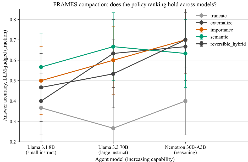
Figure 3: The smart-versus-blind gap widens with capability on FRAMES (EXP-003c). Every structure- or retrieval-preserving arm climbs from the 8B to the reasoning model while blind truncation stays at the floor, so the distance grows from about 0.2 to about 0.3.
