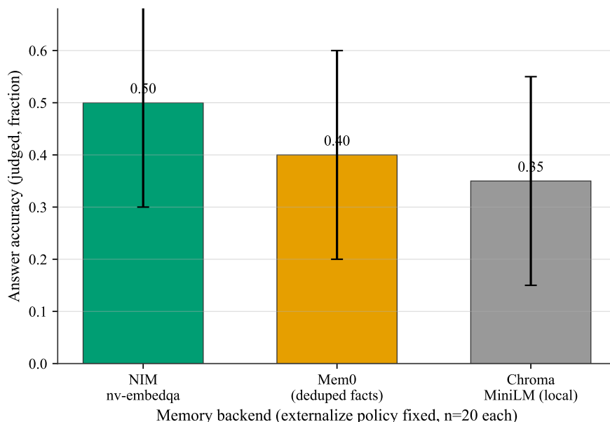
Figure 6: Under a fixed externalize policy, the memory backend is the lever (EXP-006). The same FRAMES questions through the same policy: a retrieval-tuned embedder (NIM nv-embedqa) leads, a general local one (Chroma MiniLM) trails, and Mem0’s extract-then-dedupe distillation sits between, n=20 each with the wide intervals shown.
