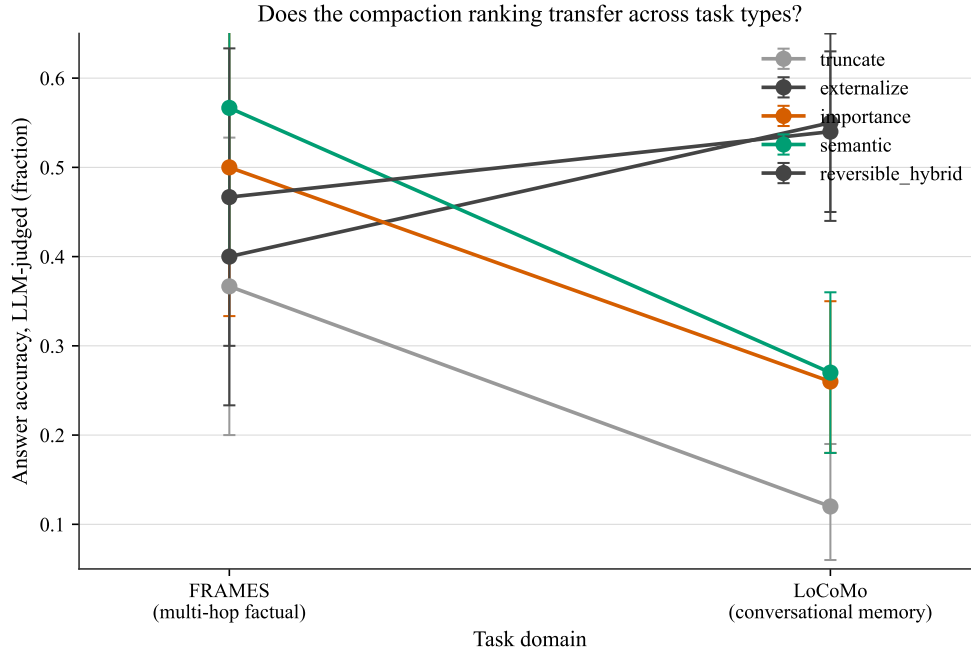
Figure 4: The compaction-policy ranking inverts across domains (EXP-004). Summary policies (semantic, importance) lead on factual FRAMES and collapse on conversational LoCoMo, where the retrieval policies (externalize, reversible hybrid) lead instead.
