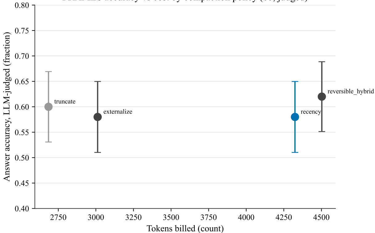
FRAMES accuracy vs cost by compaction policy (8b, judged)
