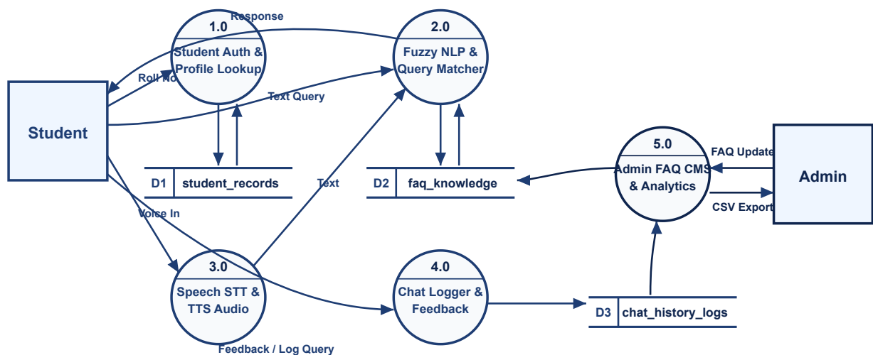
DFD Level 1: Process Decomposition
