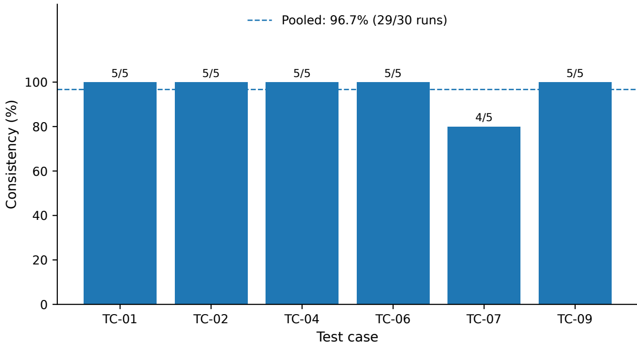
Recommendation consistency over 5 repetitions on identical evidence
