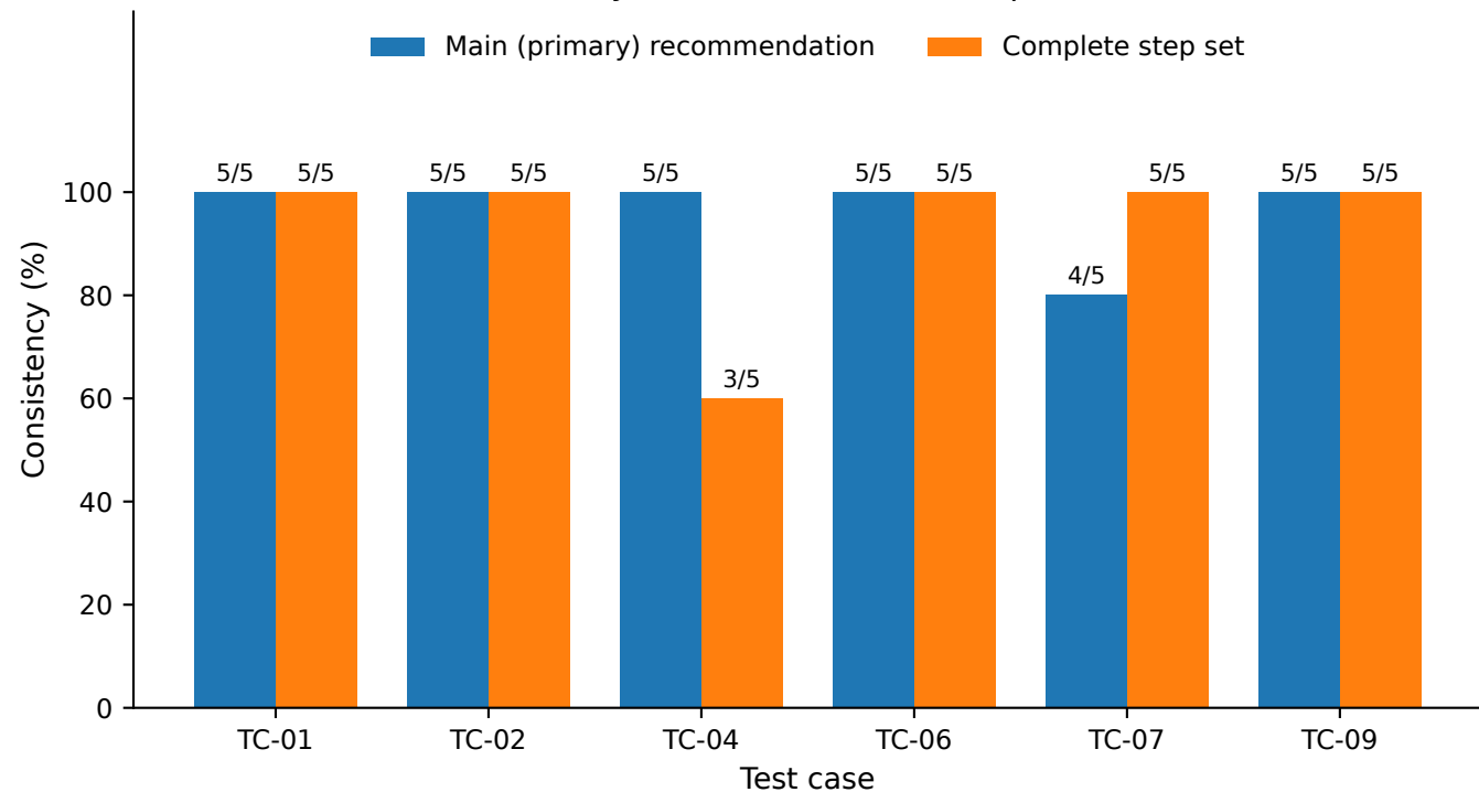
Recommendation consistency on identical evidence (pooled main 96.67%, 29/30)
