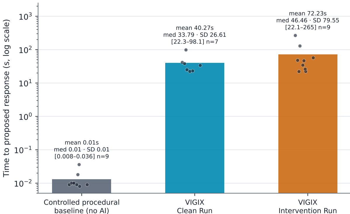
Figure 3 Investigation time: baseline vs VIGIX
