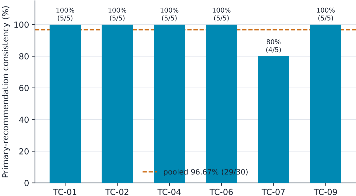
Figure 4 Recommendation consistency (5 repetitions on identical evidence)
