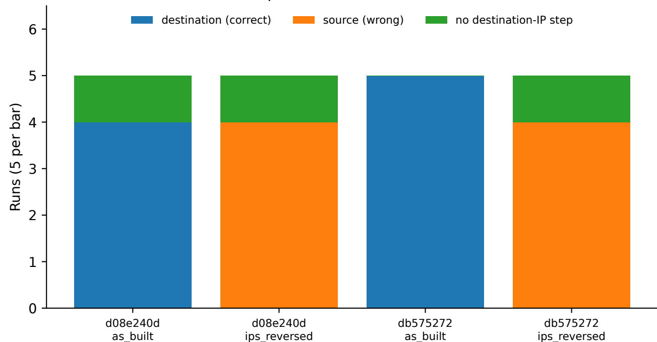
First destination-IP step vs the order of IP candidates in the context
