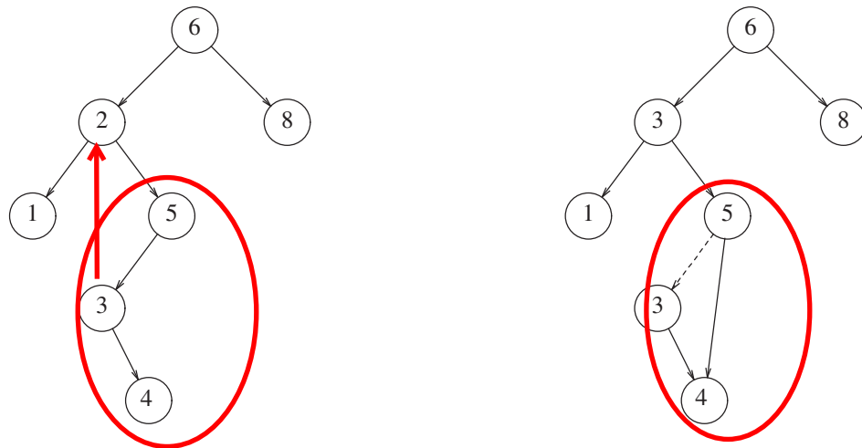
Figure 4.25 Deletion of a node (2) with two children, before and after
