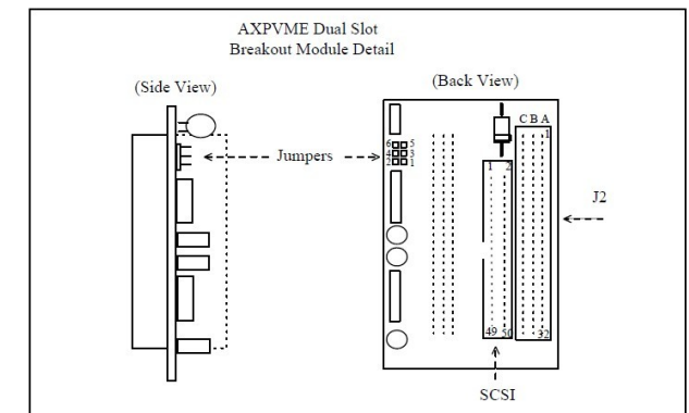
Figure 1-80 AXPvme Dual-Slot Breakout Detail
