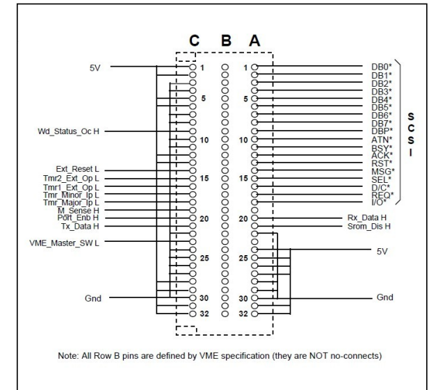
Figure 1-80 AXPvme Dual-Slot Breakout Detail
