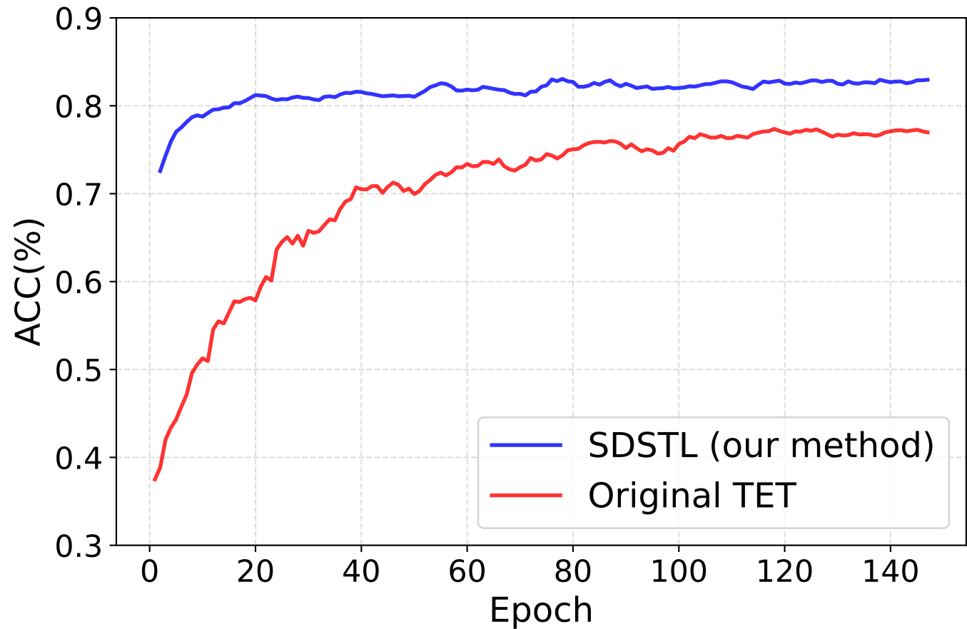
Comparison of SDSTL and Original TET on DVS-CIFAR10
