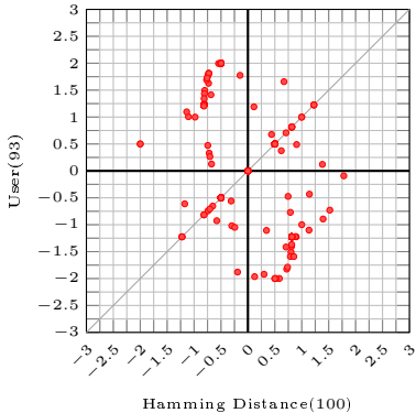
Score Z-Score Normalized 315/327
