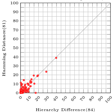
Score Deviation from Original 314/327
