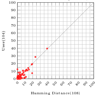
Score Deviation from Original 318/327
