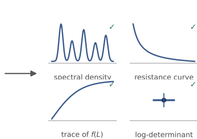
CLASSICAL · RE-READ AT NO QUANTUM COST
