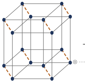
INPUT: IMPLICIT OPERATOR succinct rule, never stored signed edges dashed
