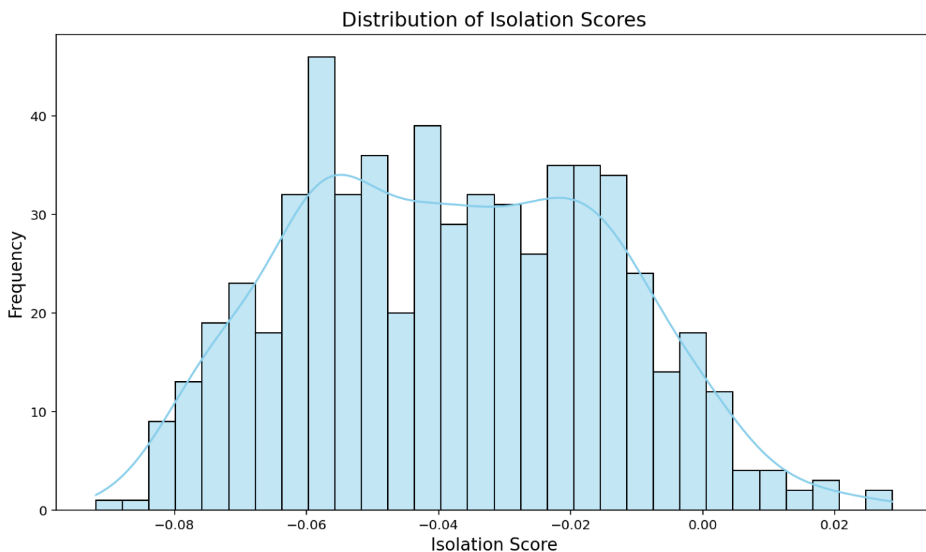
Figure: Distribution of Isolation Forest anomaly scores. Right-tail samples correspond to stronger bias signals.
