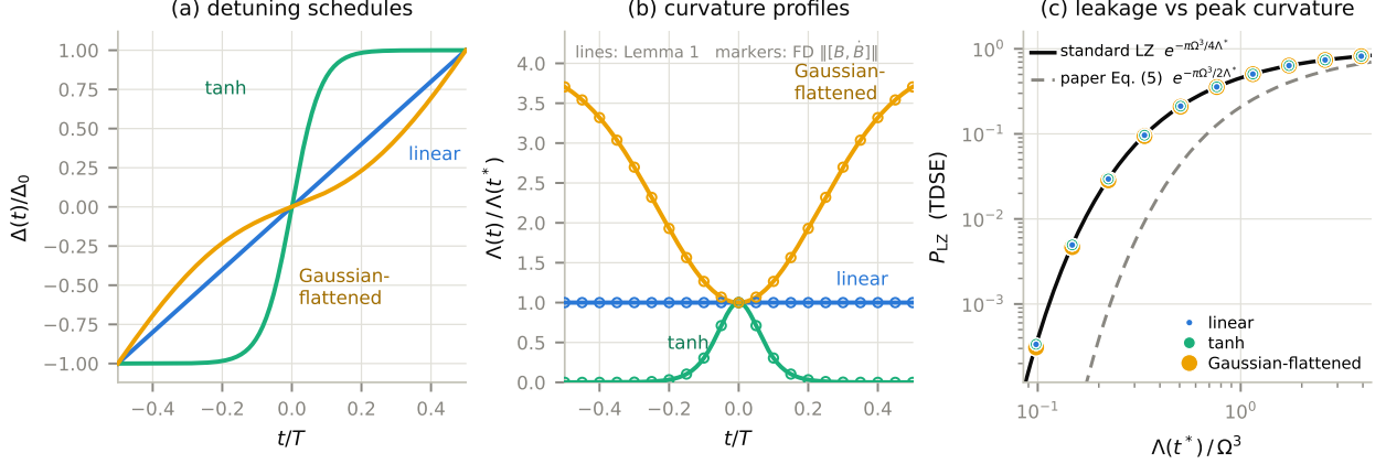
Figure 1: Curvature sweeps. (a) The three detuning schedules (representative runs, \Omega = 1 ). (b) Curvature profiles \Lambda(t)/\Lambda(t^*) : lines are the Lemma 1 identity \frac{1}{2}\Omega|\dot{\Delta}| ; markers are the independent finite-difference evaluation of \|[B, \dot{B}]\| (agreement < 4 \times 10^{-9} relative). (c) Measured leakage versus normalized peak curvature for all 90 runs (3 schedules \times 3 values of \Omega \times 10 ramp rates; markers are nested by size because the three schedules land on the same points, and the three \Omega branches coincide to < 10^{-12} relative—the exact scale invariance underlying the \Lambda(t^*)/\Omega^3 collapse). The solid curve is Eq. (5), \exp(-\pi\Omega^3/4\Lambda(t^*)) , which the data follow; the dashed curve is the constant printed in earlier drafts, \exp(-\pi\Omega^3/2\Lambda(t^*)) , retained for comparison (corrected in this revision).
