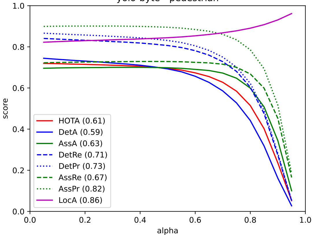
yolo-byte - pedestrian
