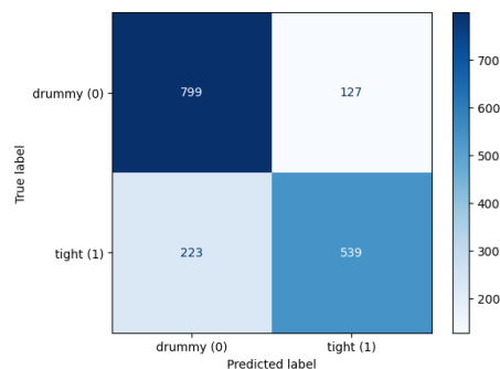
Figure 9: Phase 2 PCA Best Confusion Matrix
