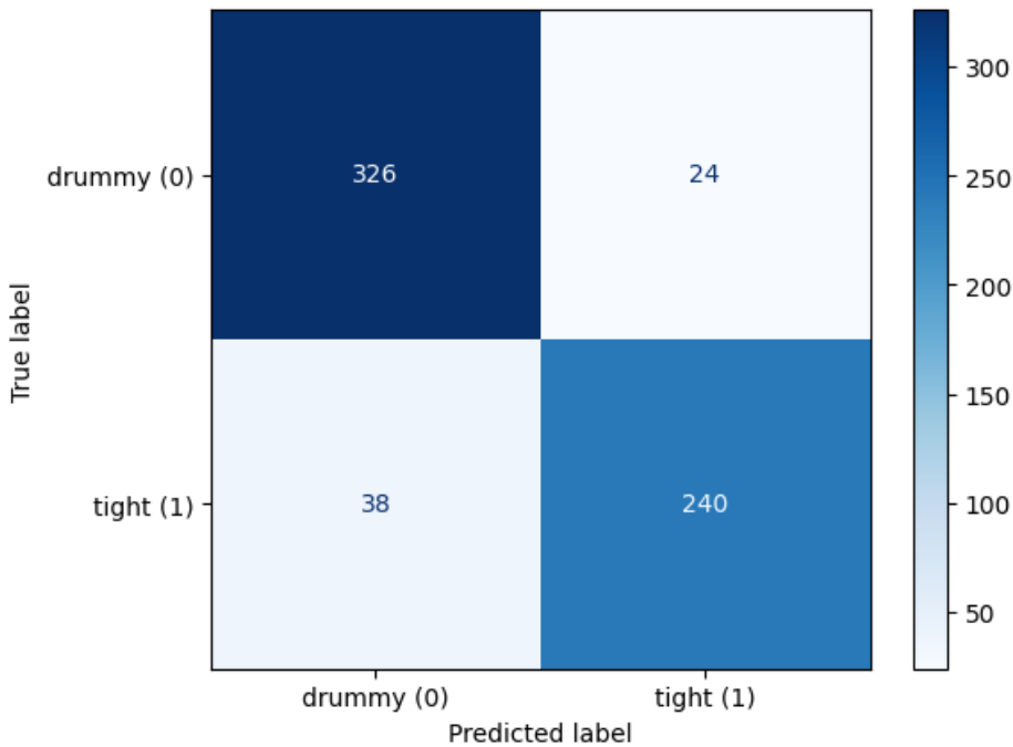
Figure 21: MFCC MLP Confusion Matrix (Phase 2)
