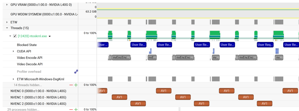
Fig. 1: Nsight Systems timeline view displaying Video Encode API and dedicated NVENC hardware engine rows.
