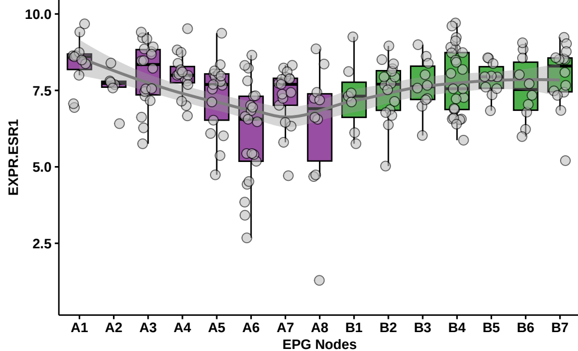
Trajectory: A-B (trend: p=0.92116 )
