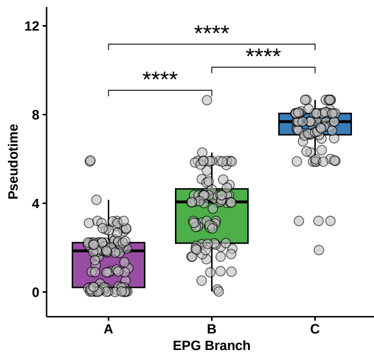
EPG Branches (trend: p=0.29627 )
