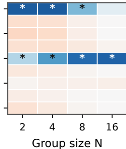
(b) CIFAR-100
