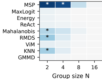
(a) CIFAR-10
