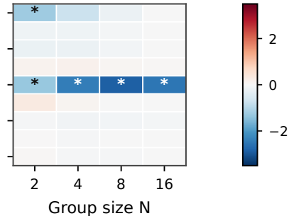
(c) ImageNet-200
