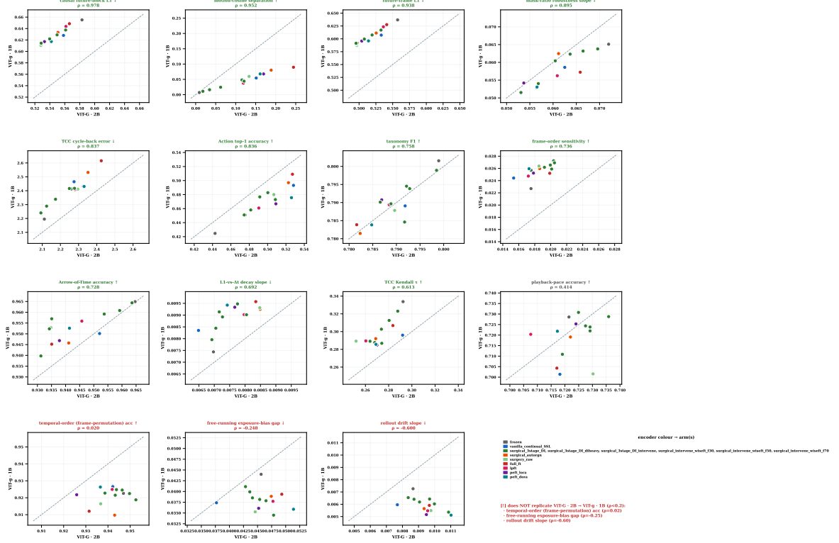
Figure 5: Complete cross-scale ranking robustness (2B→1B), all fifteen diagnostics. Each panel plots per-method scores at the V-JEPA 2.1 (2B) scale ( x ) against the V-JEPA 2.1 (1B) scale ( y ); the dashed line is the identity y = x . Panels are sorted by Spearman rank correlation \rho (descending): green titles mark strong replication ( \rho \geq 0.5 ), grey inconclusive ( 0.2 \leq \rho < 0.5 ), and red failure ( \rho < 0.2 ). Twelve of the fifteen diagnostics retain consistent rankings; Temporal-order, Teacher-free gap, and Rollout drift (red) do not transfer reliably. The strongest-replicating panel, Causal future-block L1 ( \rho = 0.978 ), is featured in the main paper.
