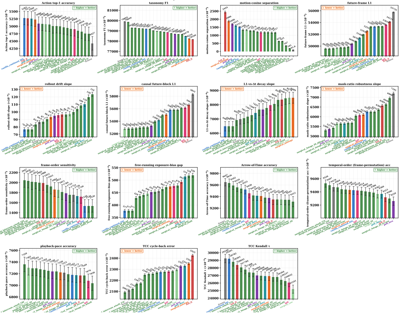
Figure 4: Complete V-JEPA 2.1 (2B) attribution and ablation scorecard. The comparison includes frozen and continually adapted V-JEPA, full and parameter-efficient fine-tuning, Auto-RGN, FactorJEPA-RAW, the executed FactorJEPA objective variants, and the WiseFT encoder-scope variants. Bars report held-out means; error bars denote 95% BCa confidence intervals where available. Each panel states whether higher or lower values are preferred. Internal variants are mapped to their publication-facing definitions in Table 6. Attribution claims use the prespecified contrasts in the prespecified contrasts, rather than selecting the best method separately for each diagnostic.
