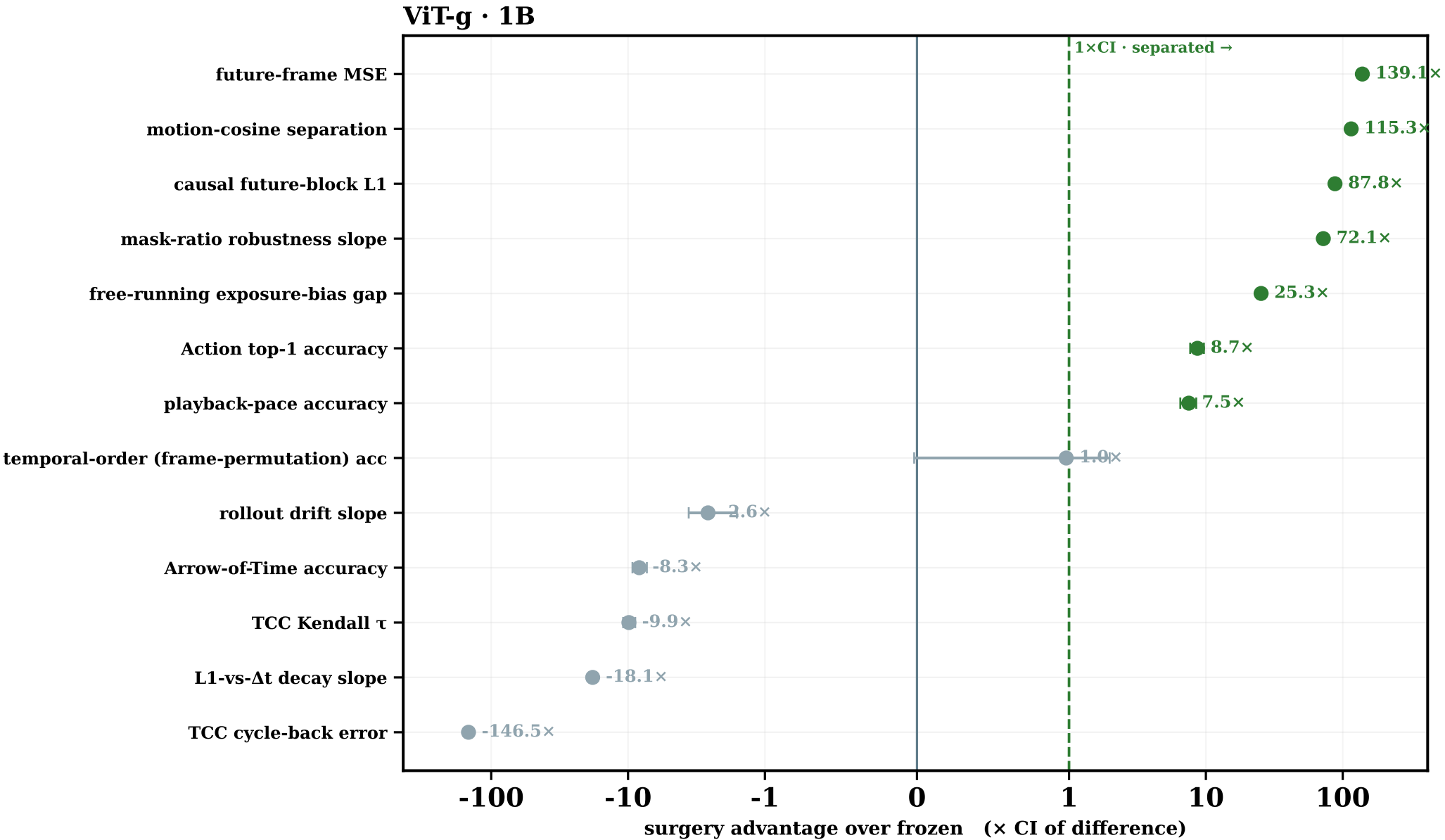
Forest plot — does surgery statistically separate from frozen? (green past dashed line = yes · surgery_raw ∈ OURs)
